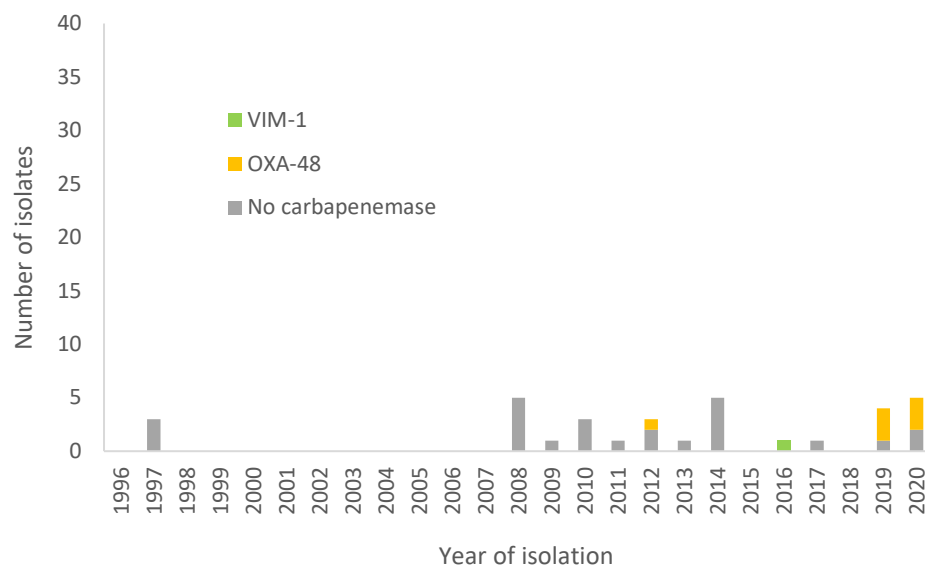
Figure 4. Number of hypervirulent K. pneumoniae (hvKp) ST23 isolates with and without carbapenemase genes in the main clade, EU/EEA, n=33*†
