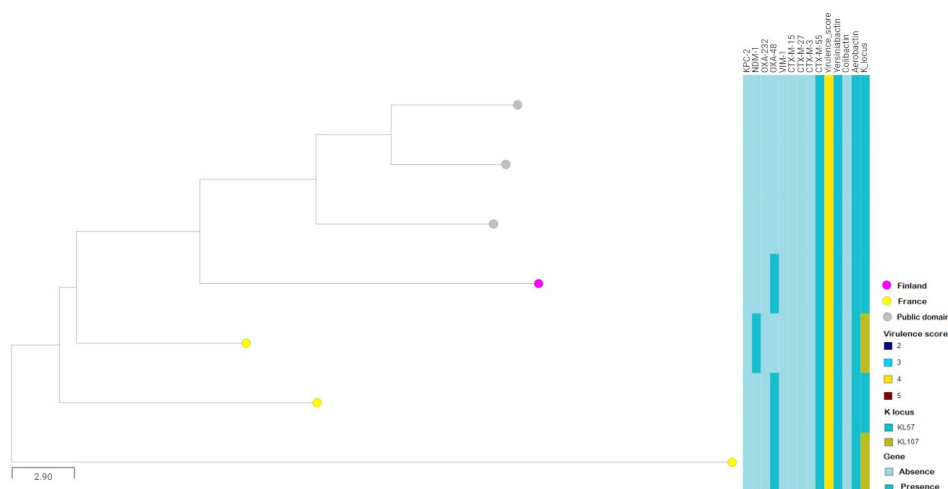
Figure 5. Separate clade with neighbouring relationships of hypervirulent Klebsiella pneumoniae (hvKp) ST23 isolates submitted for this study (coloured by country) and from open-access databases (grey) (n=7)
