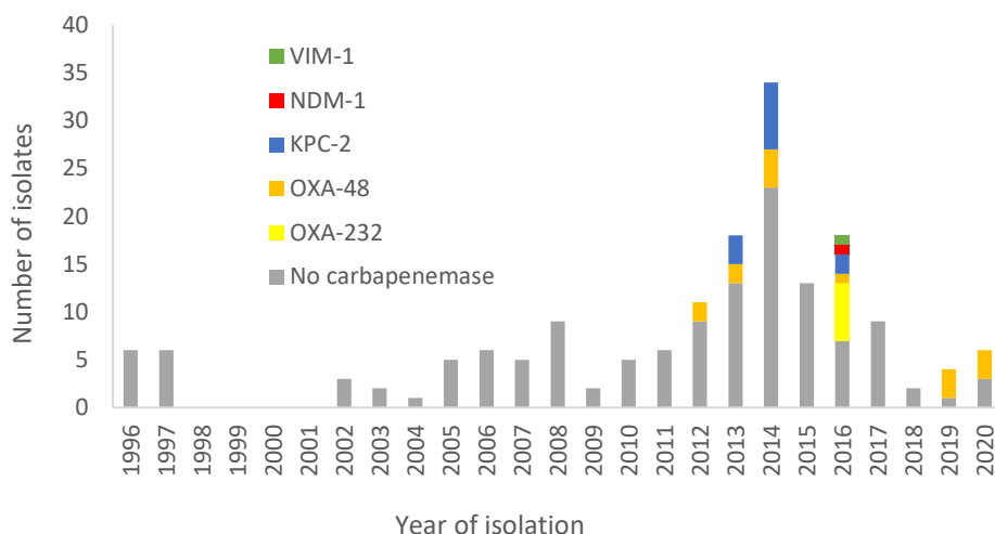
Figure 3. Number of hypervirulent K. pneumoniae (hvKp) ST23 isolates with and without carbapenemase genes in the main clade, worldwide, n=171*†
