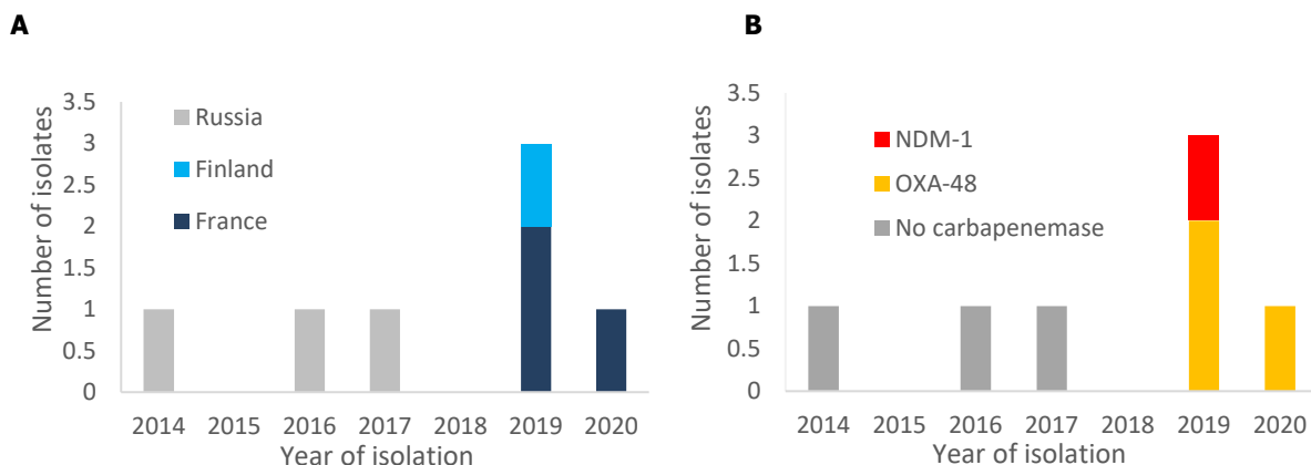
Figure 6. Number of cases of hypervirulent K. pneumoniae (hvKp) ST23 isolates in the separate clade, (A) by country and (B) presence of carbapenemase (n=7)
